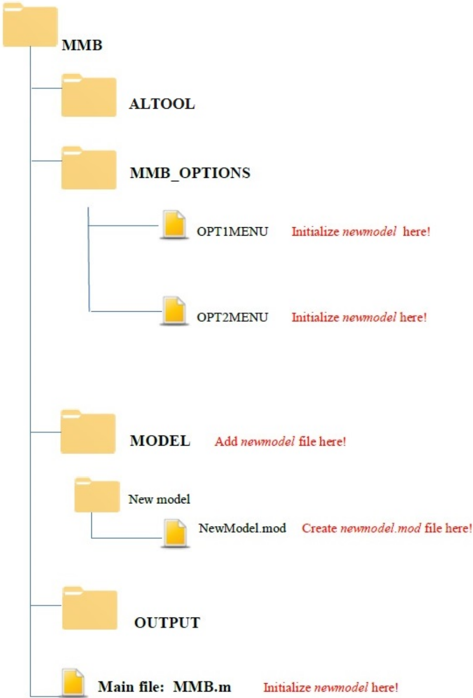
Figure 13: ADDING MODELS IN THE MODELBASE
